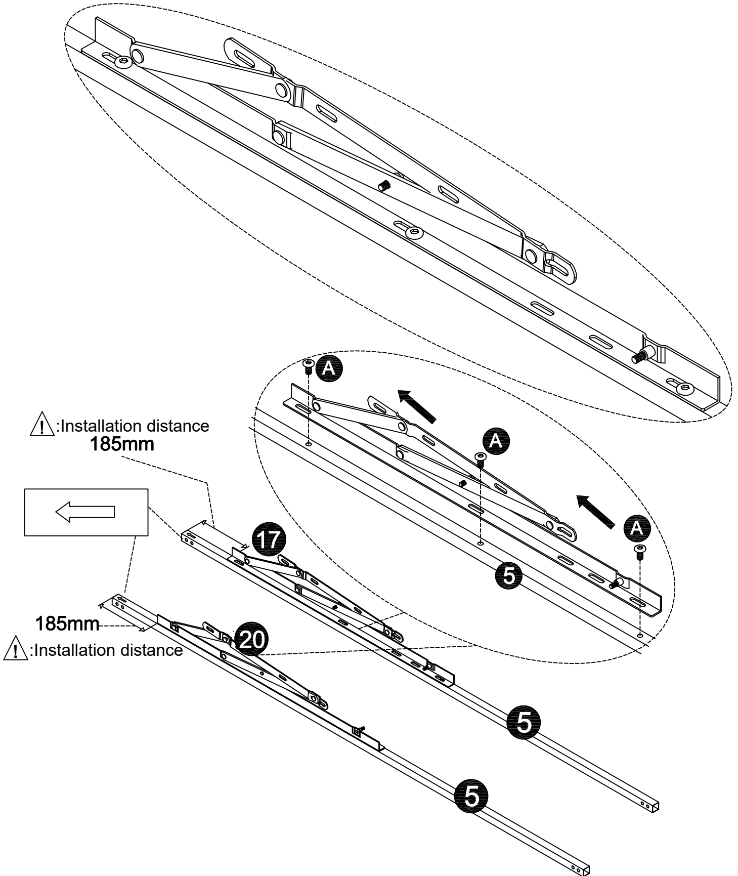
Installation position diagram
